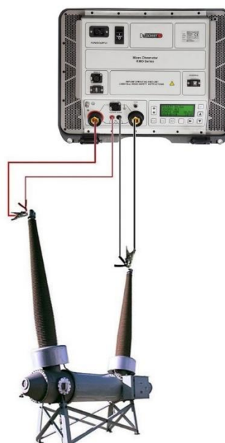
RMO-G cable connection on dead tank circuit breaker
