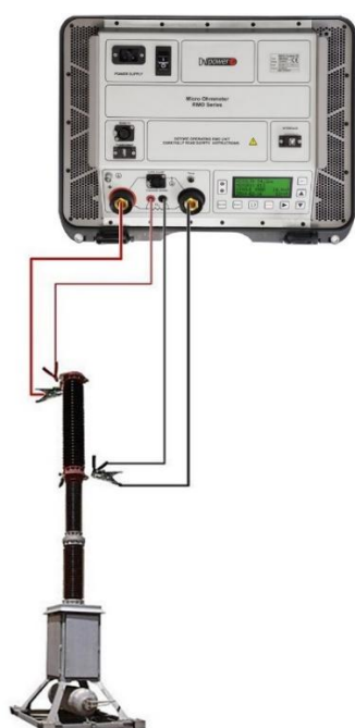
RMO-G cable connection on live tank circuit breaker
