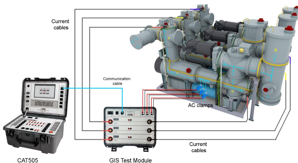
Timing measurement of single pole controlled GIS under BSG conditions with use of GIS Test Module
