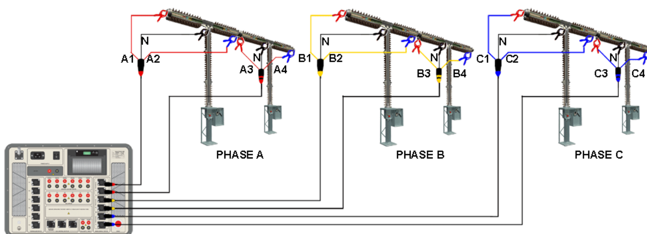
Conventional timing measurement – main contact timing cables connection to a live tank circuit breaker (4 breaks per phase)
